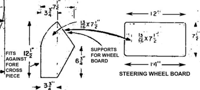
STEERING WHEEL SUPPORT - 2 REQ
