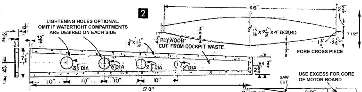
STRINGER: 2-REQ 1-RIGHT 1-LEFT
